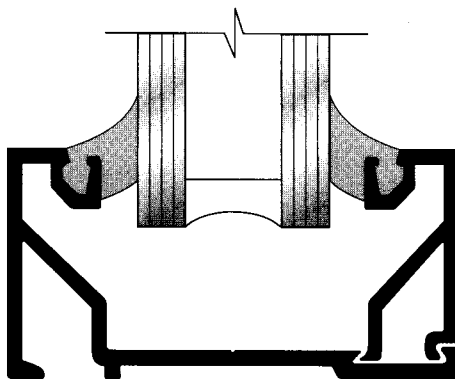
22-620T SASH Transom Condition for 1" Glazing
