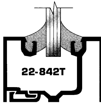
Transom Condition for 1/4" Glazing
